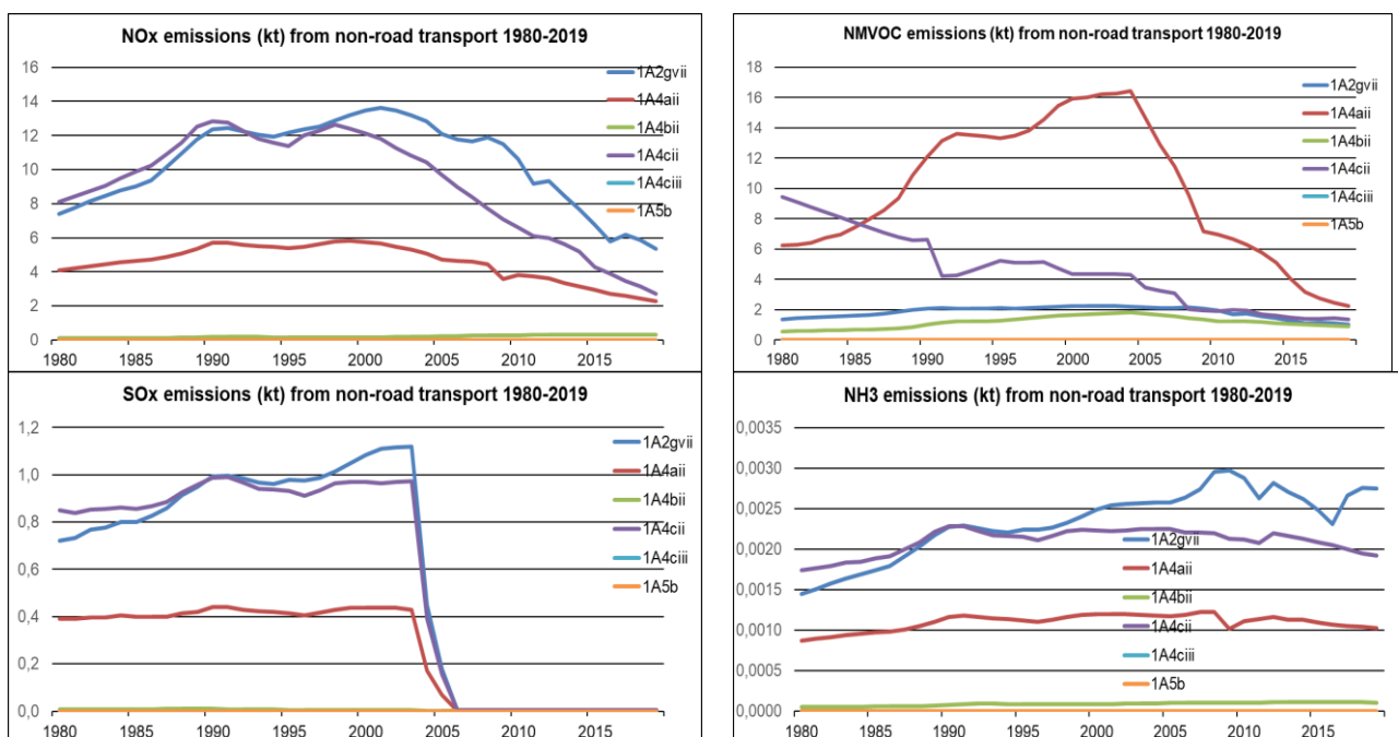
Figure 3.12 Emission trends 1980-2019
